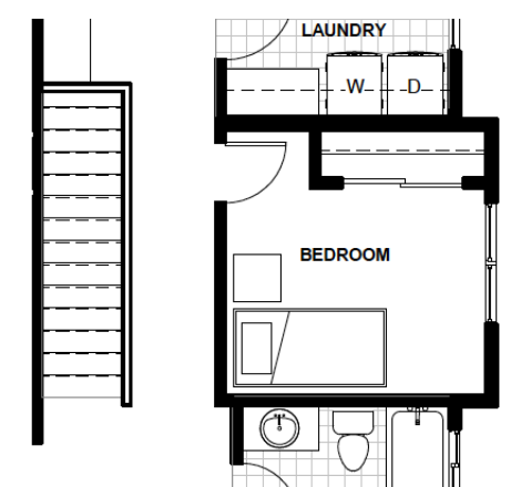
FLEX ROOM OPTION 2: BEDROOM
